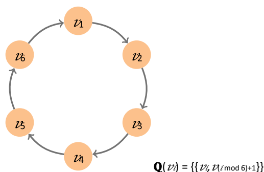
Fig. 4. Cyclic quorum structure example
