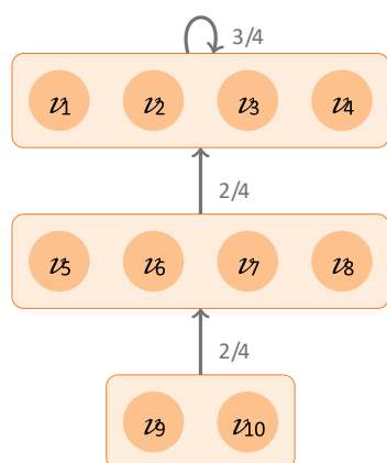
Fig. 3. Tiered quorum structure example
